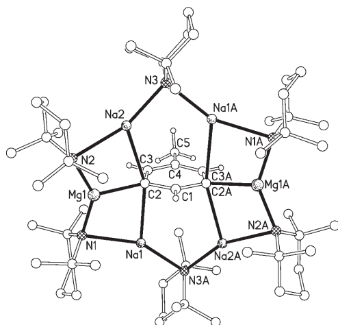
Figure 3. Molecular structure of 4 , with tmp hydrogen atoms omitted for clarity. Symmetry operator ( C_2 axis) A: -x, y, 1/2 - z . Selected bond lengths [Å] and angles[°]: Mg1–N1 2.058(3), Mg1–N2 2.053(3), Na1–N1 2.599(3), Na1–N3A 2.400(3), Na2–N2 2.570(2), Na2–N3 2.361(3), Mg1–C2 2.217(3), Na1–C2 2.801(3), Na2–C2 2.749(3); N1–Mg1–N2 101.09(10), N1–Mg1–C2 108.45(11), N2–Mg1–C2 111.07(11), N1–Na1–N3A 155.55(10), N1–Na1–C2 79.86(9), N3A–Na1–C2 123.88(9), N2–Na2–N3 159.88(9), N2–Na2–C2 82.84(9), N3–Na2–C2 117.06(9).
